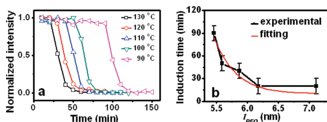
Figure 3. (a) Evolution of normalized I(q) during crystallization of PEO at 45.5 °C. The PLLA- b -PEO samples with the PLLA blocks initially isothermally crystallized at temperatures indicated in the Figure. (b) Plot of the induction time of PEO crystallization vs l_{\text{PEO}} .
